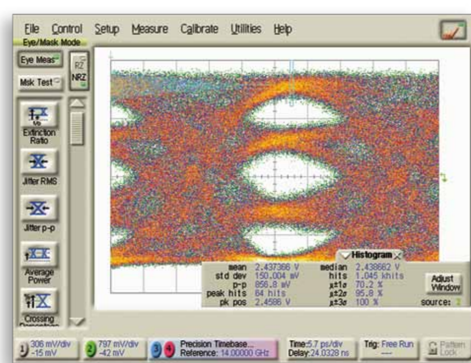
Eye Diagram: 32 Gbps
