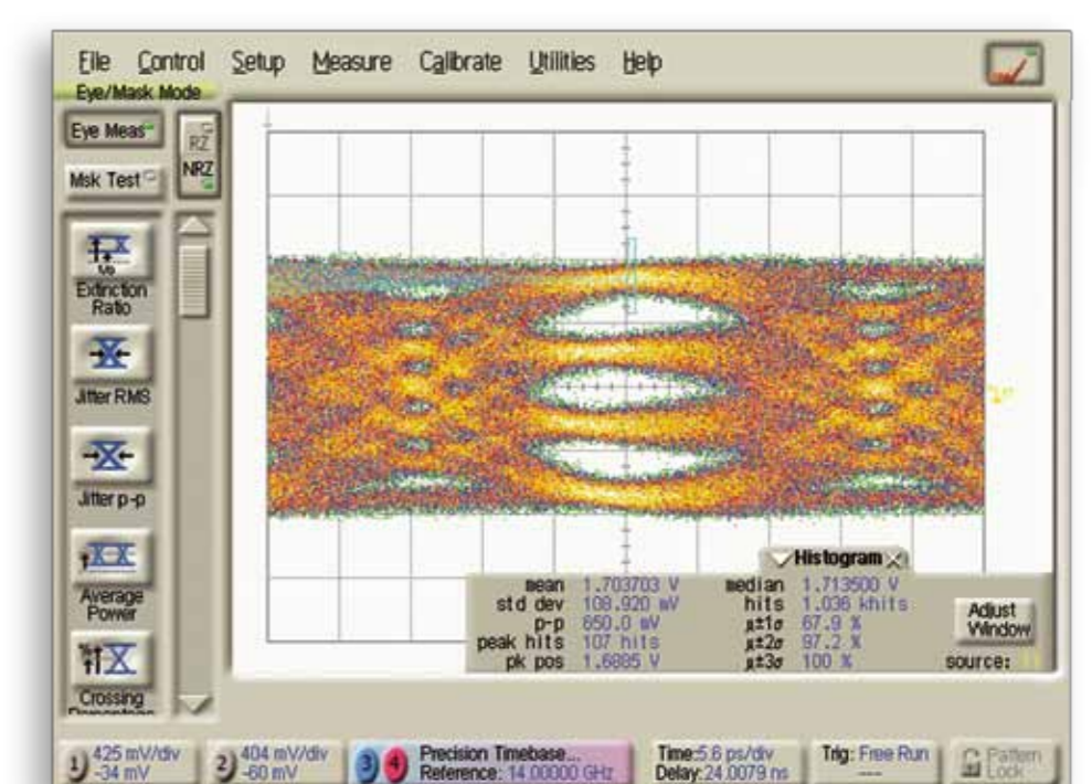
Eye Diagram: 32 Gbps
