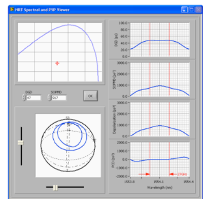
Blue shows the DGD, SOPMD, Depolarization, PDCD & PSP spectra. A red 27 GHz wide band is shown for reference.
